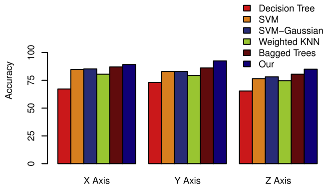
Fig. 12. Performance of algorithms using 1-axis acceleration (UCI Dataset) (Anguita et al., 2013).
