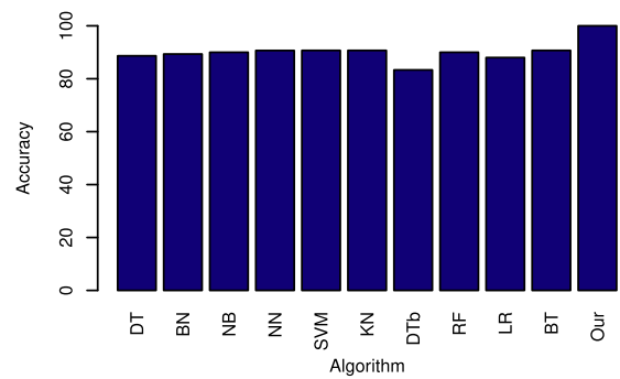
Fig. 11. Algorithm Performances using 1-Axis Acceleration (Our Dataset).
