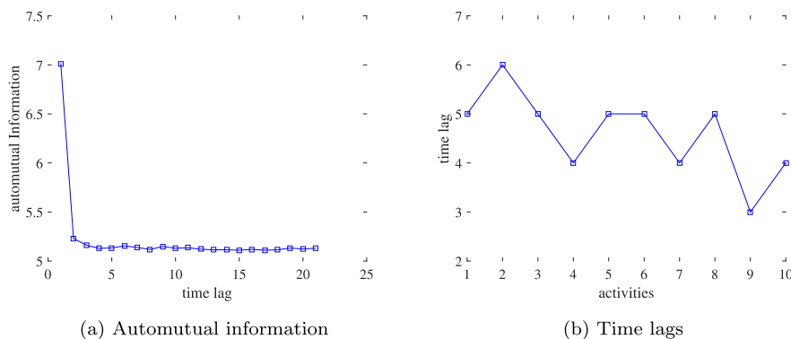
Fig. 6. Time lag estimation for walking activity.
