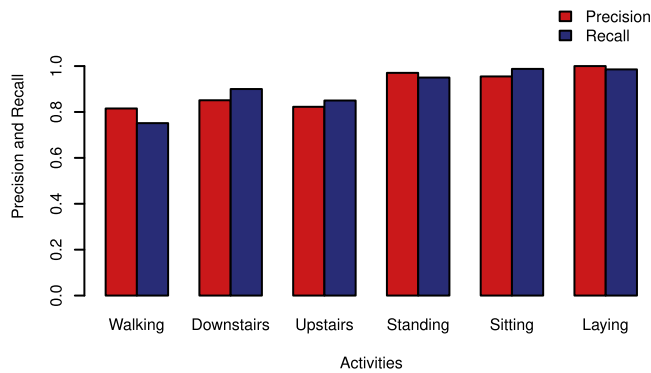
Fig. 10. Precision and recall for each activity class (Public Dataset).
